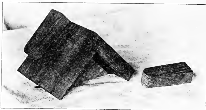
FIG. 544. STOP-OFF CORE-PRINT.
